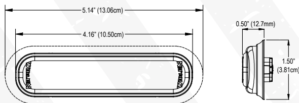
Flange Dimensions
